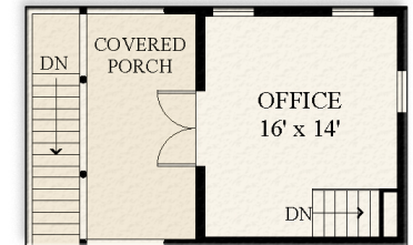
SECOND FLOOR ABOVE GARAGE
